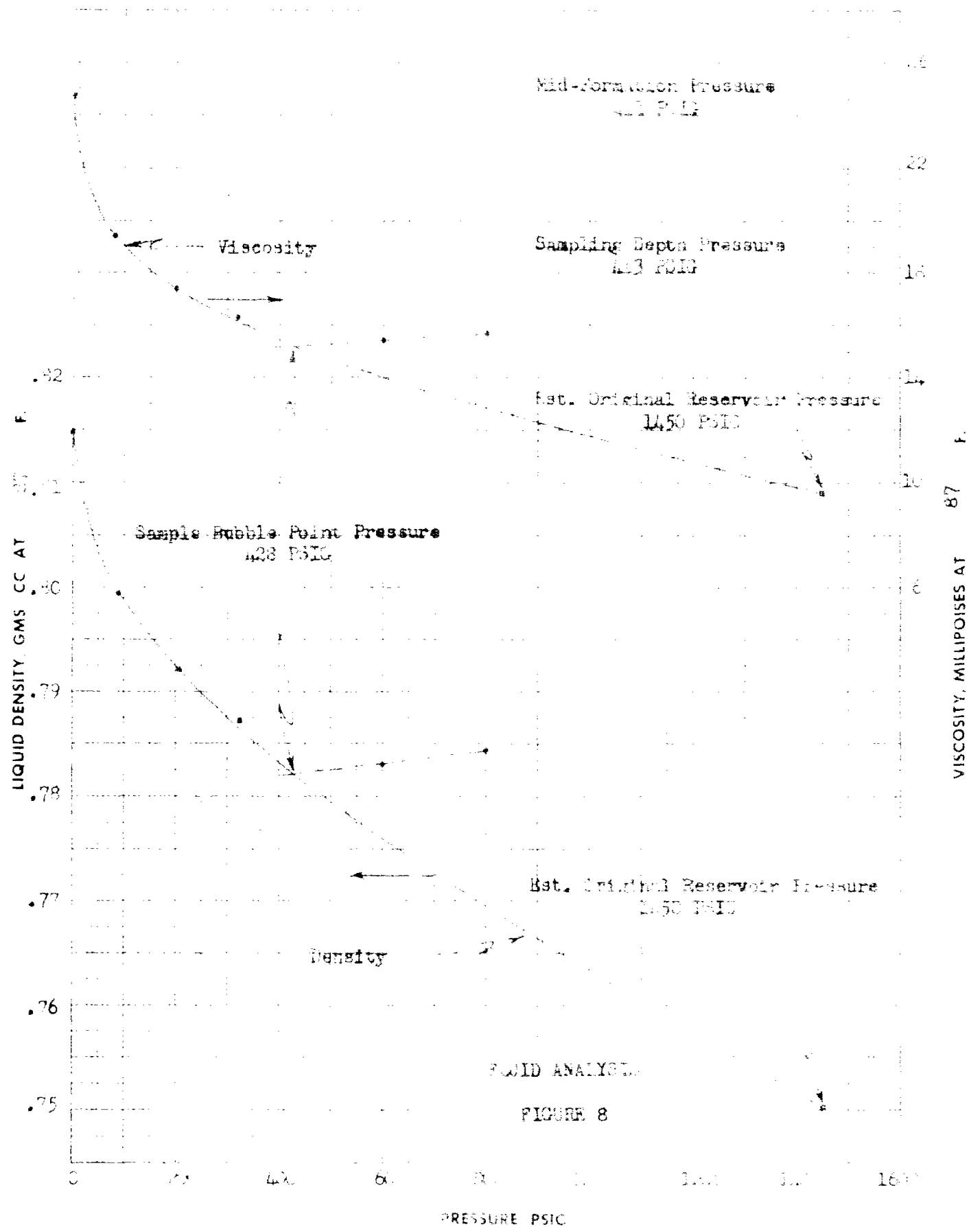
VISCOSITY - DENSITY DATA
