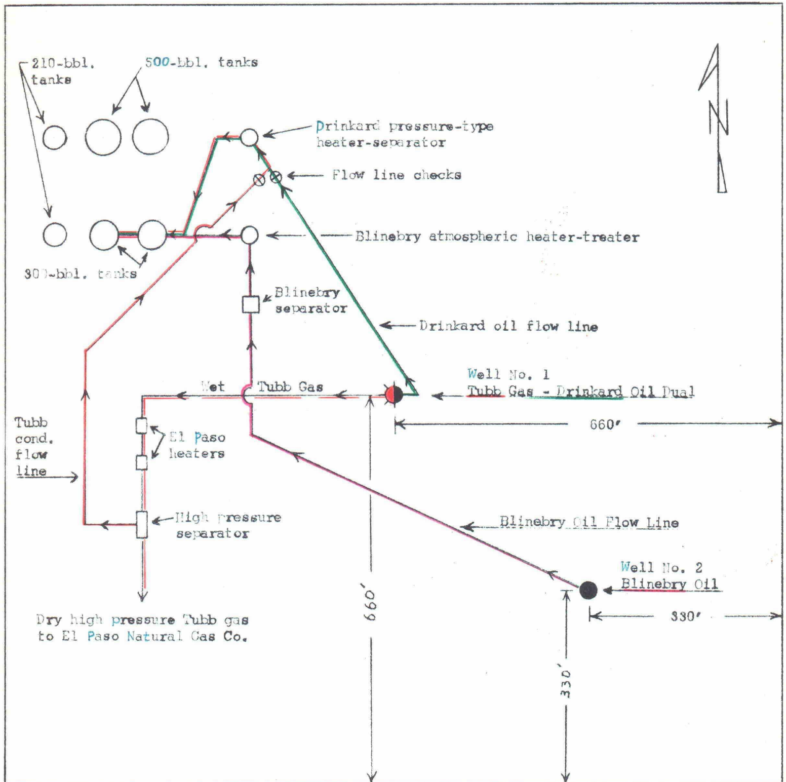
Schematic Sketch of J. R. CONE Anderson Lease NF/4 SE/4 Section 21, T-21-S, R-37-E Showing All Wells And Battery Facilities To Accompany Application For Authority To Commingle Without Separate Measurement Blinebry Oil, Drinkard Oil & Tubb Condensate
