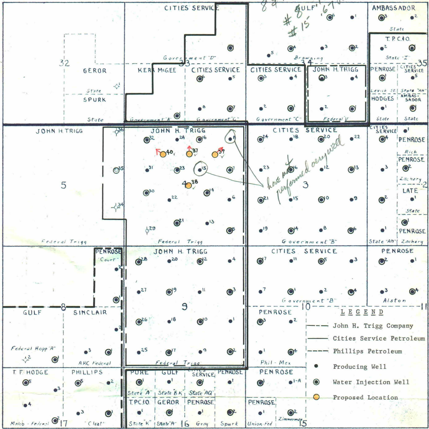
A PORTION OF THE CAPROCK QUEEN FIELD CHAVES COUNTY NEW MEXICO
