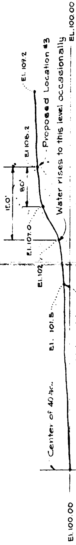
SECTION A-A Horizontal Scale 1"=100' Vertical Scale 1"=10'
