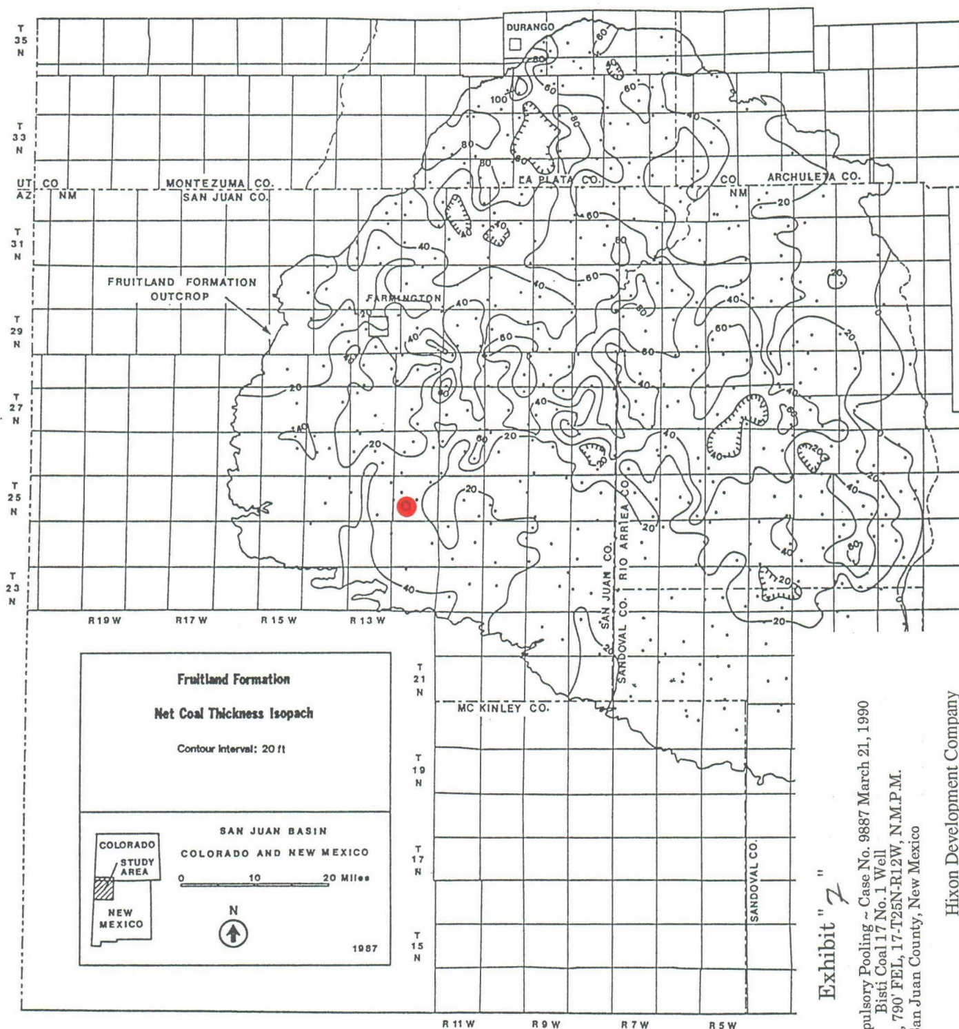
Figure 5. Fruitland Formation net-coal-thickness isopach map.
