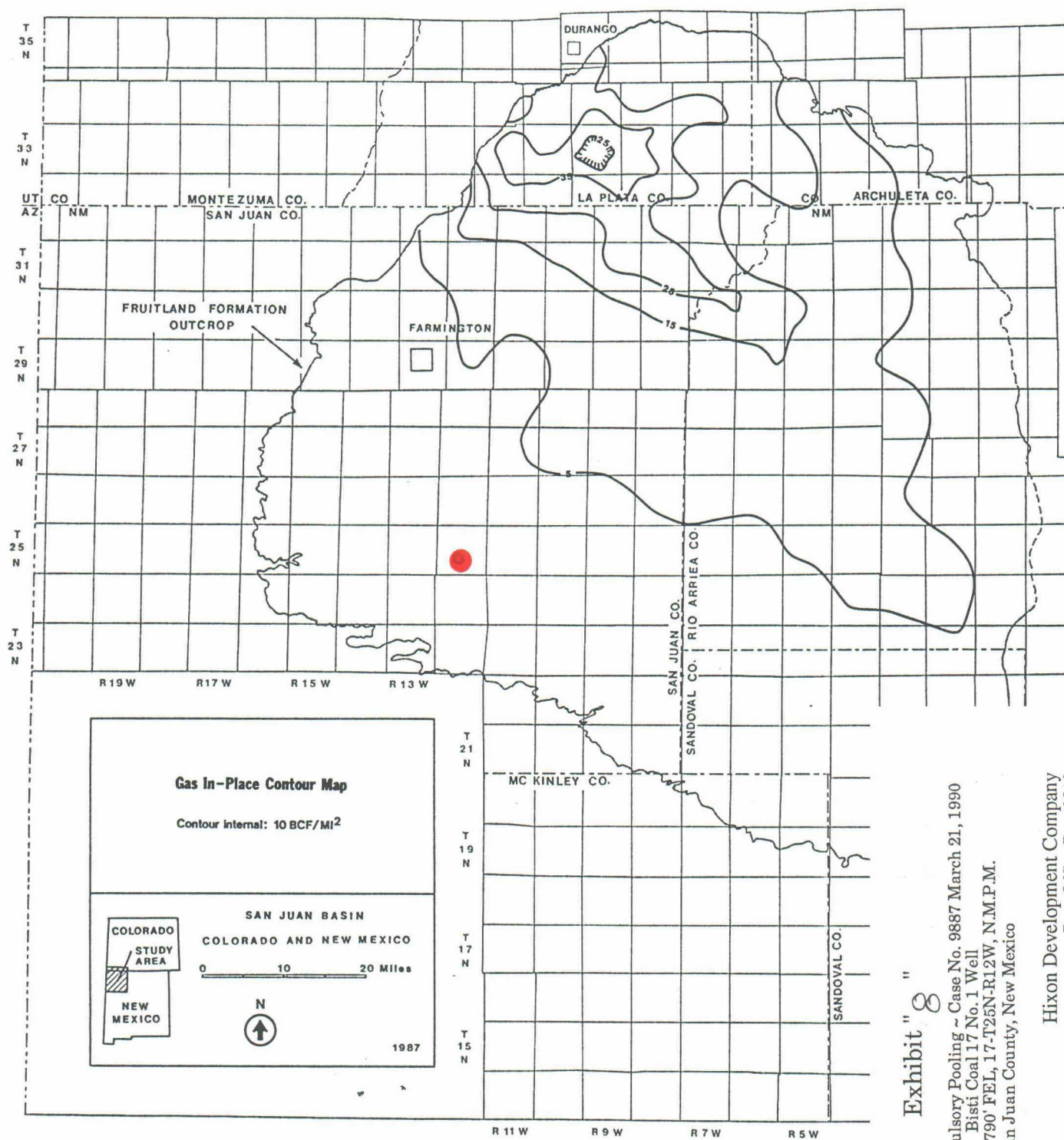
Figure 6. Gas-in-place contour map.
