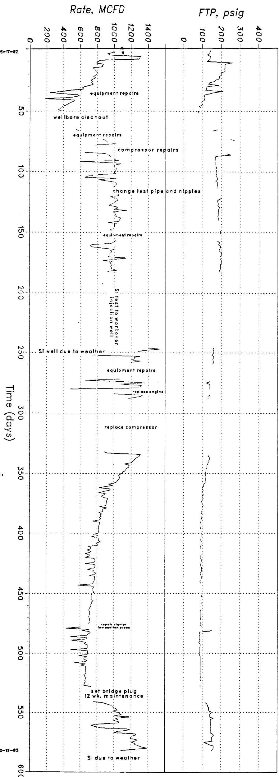
LONG-TERA FLOW TEST BDCDGU Well No. 1933 031M
