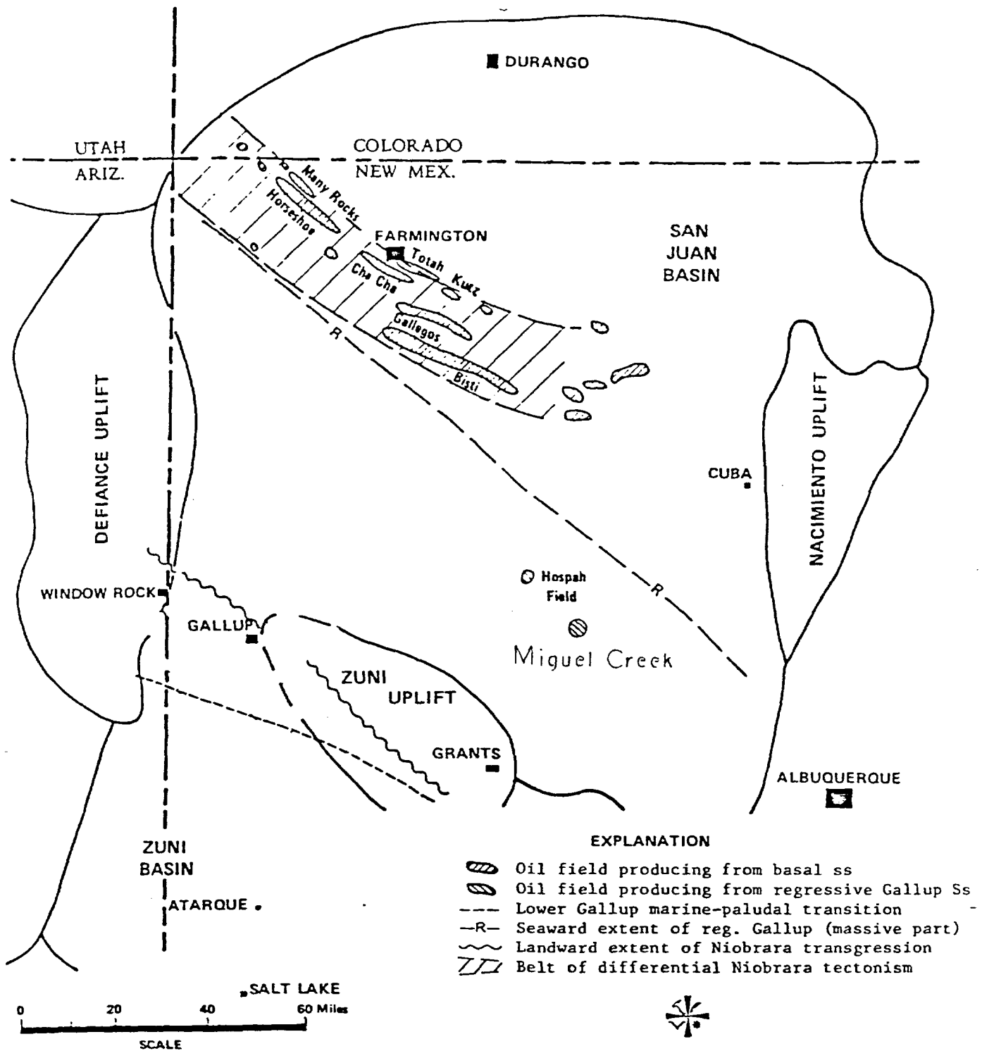
Figure 3—Producing Gallup oil fields of the San Juan Basin, New Mexico. (Modified from Molenaar, 1973.)
