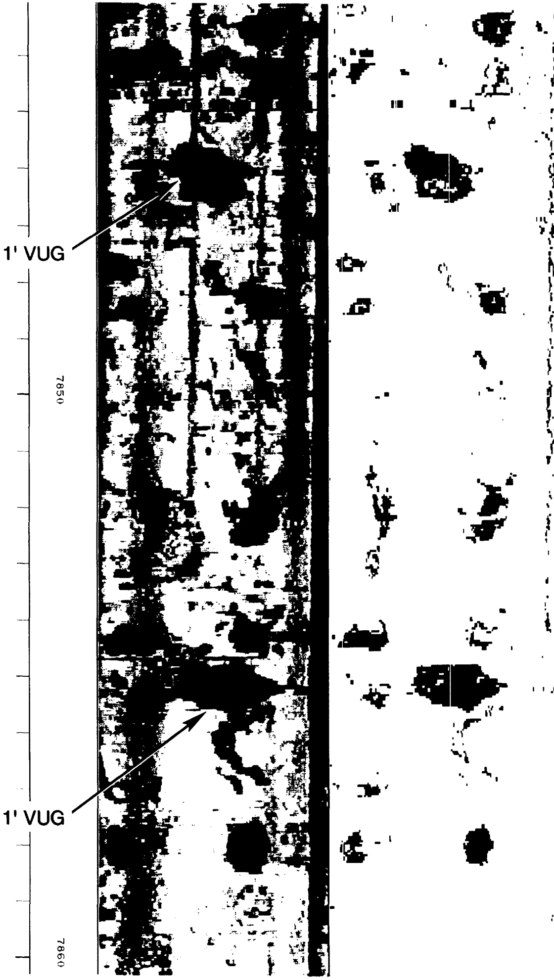
Imaging Log in Dolomite Indicating Vugular Porosity
