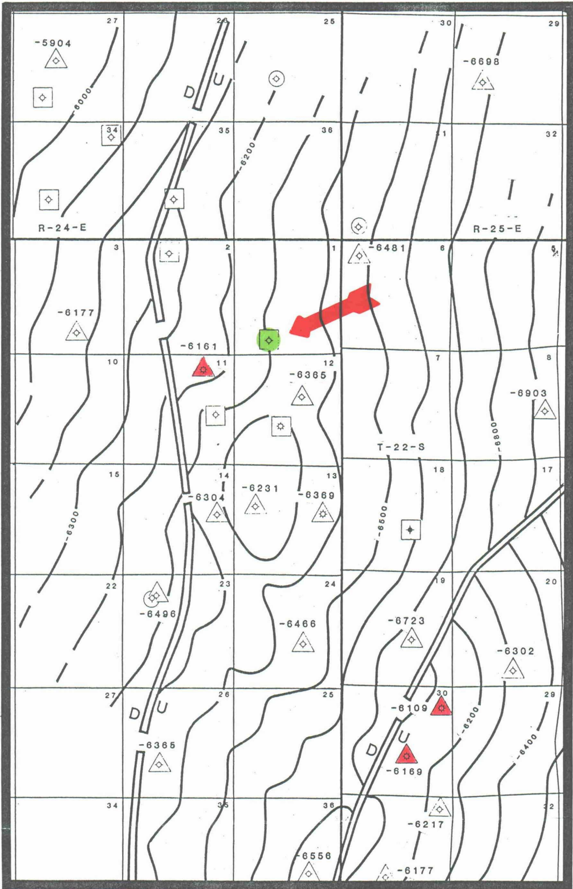
STRUCTURE, T/MIDDLE MORROW C.I.: 100 FT.
