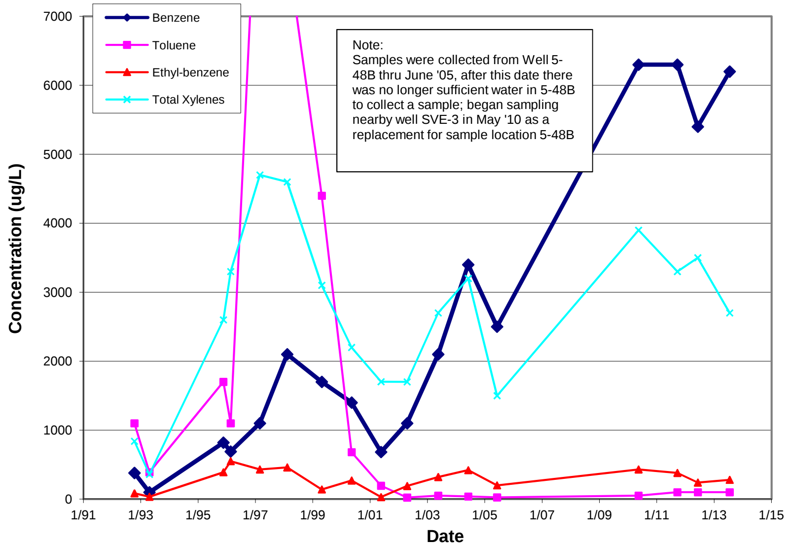
Figure 7 Concentration History at Wells 5-48B & SVE-3 TW Thoreau Station Remediation Site
