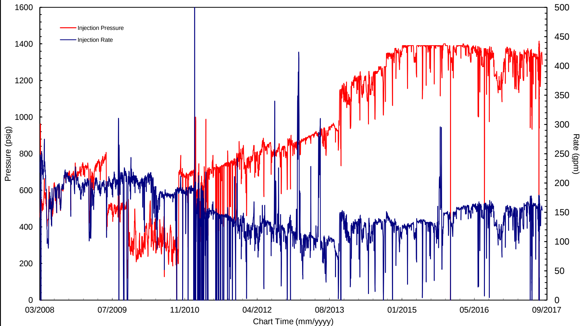
Gaines Well No. 3 Cartesian Plot of Surface Pressure and Injection Rates March 1, 2008 to August 28, 2017
