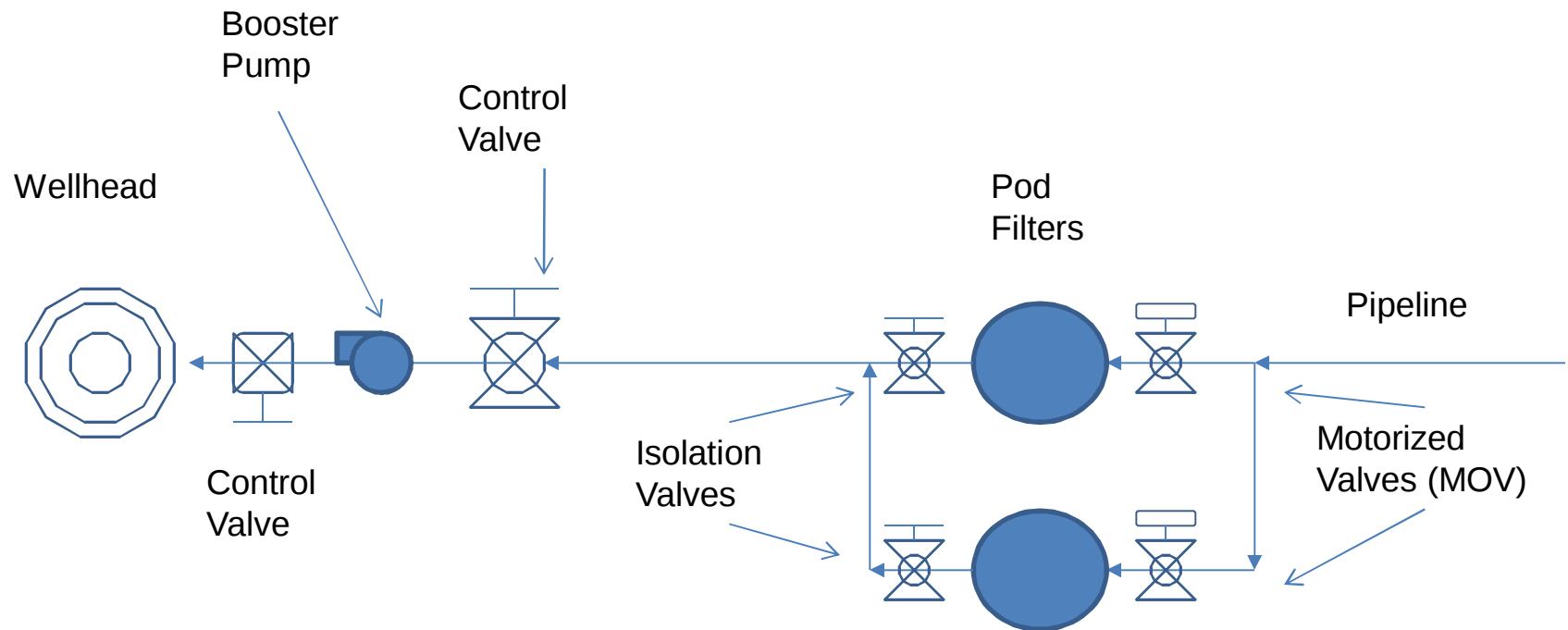
FIGURE 6 Gaines Well No. 3 Diagram of Shut-in Valve Control
