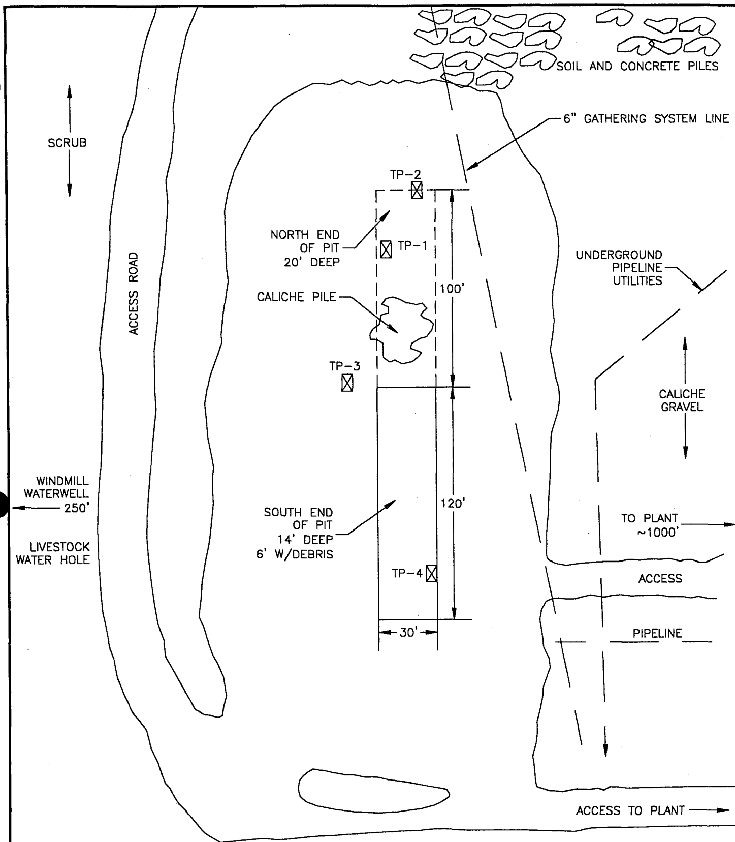
FIGURE 2 SITE MAP DUKE ENERGY FIELD SERVICES, LP ARTESIA PLANT PIT CLOSURE ARTESIA, NEW MEXICO
