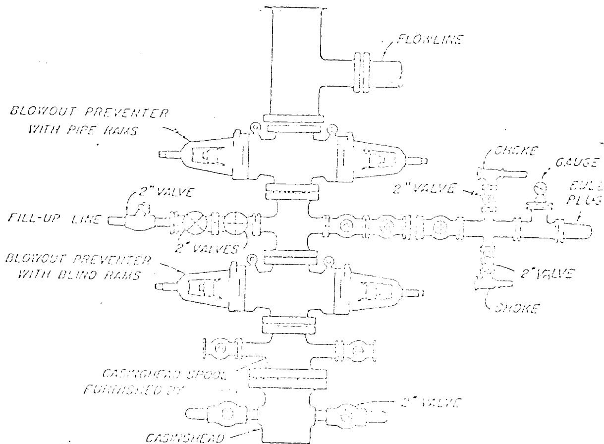
BLOWOUT PREVENTER HOOK-UP AMOCO REG. U.S. PAT. OFF.
