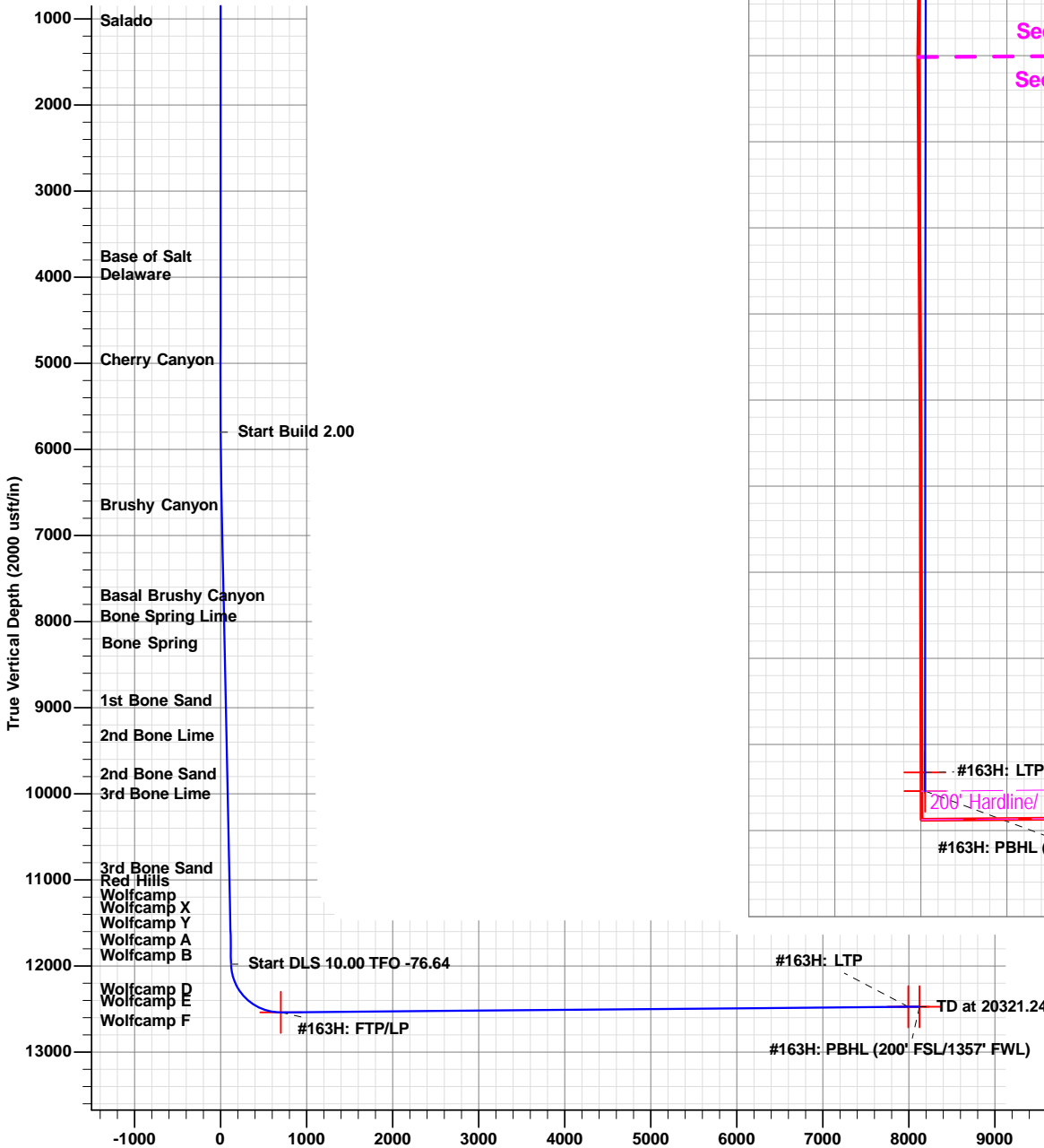
Vertical Section at 180.05° (2000 usft/in)
