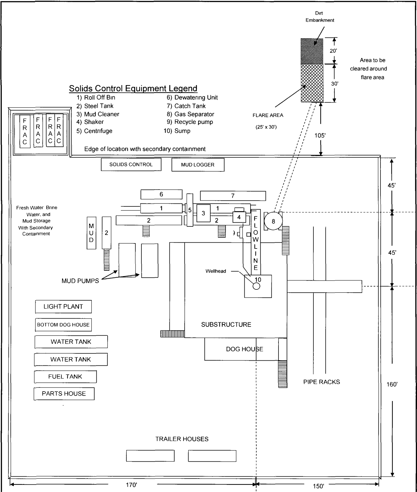
POKER LAKE UNIT 327H TYPICAL RIG LAYOUT SCHEMATIC INCLUSIVE OF CLOSED-LOOP DESIGN PLAN
