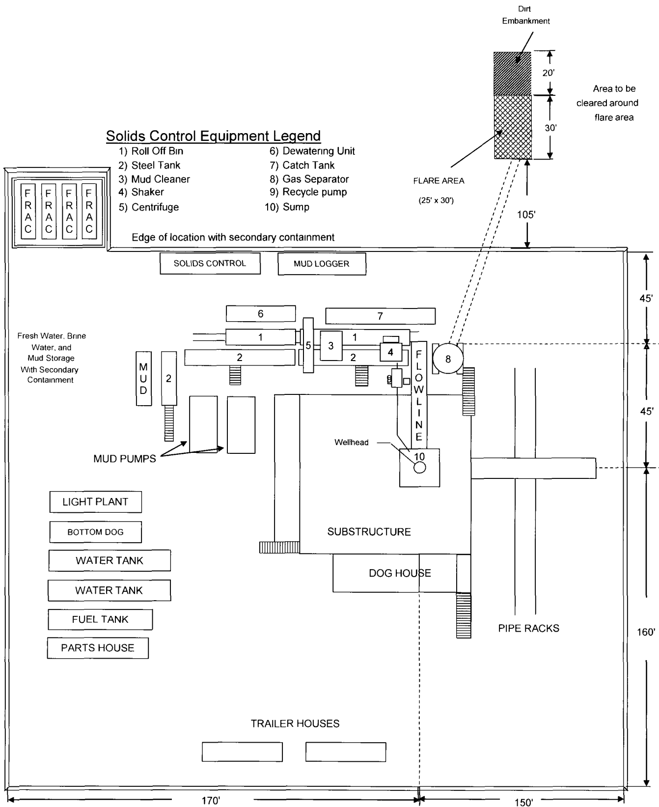
POKER LAKE UNIT 326H TYPICAL RIG LAYOUT SCHEMATIC INCLUSIVE OF CLOSED-LOOP DESIGN PLAN
