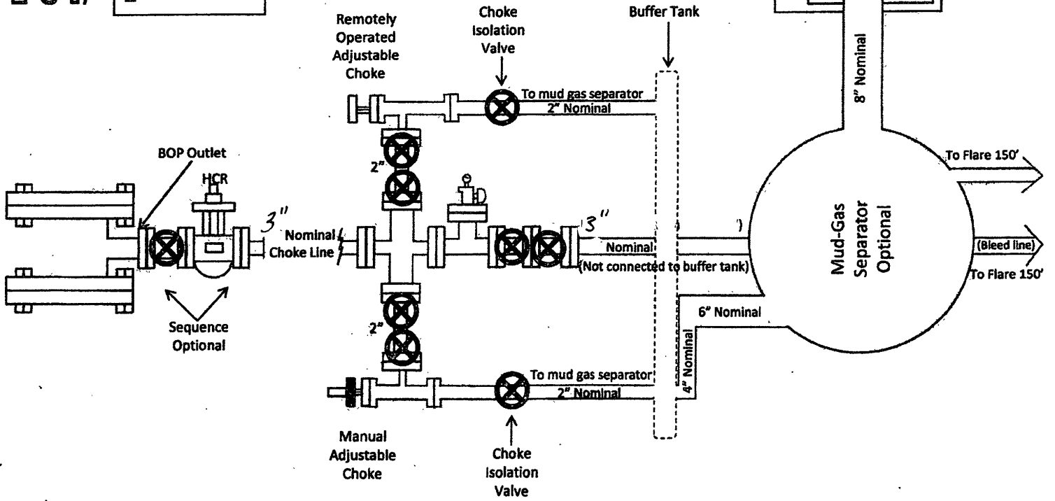
Exhibit E-1 - Choke Manifold Diagram
