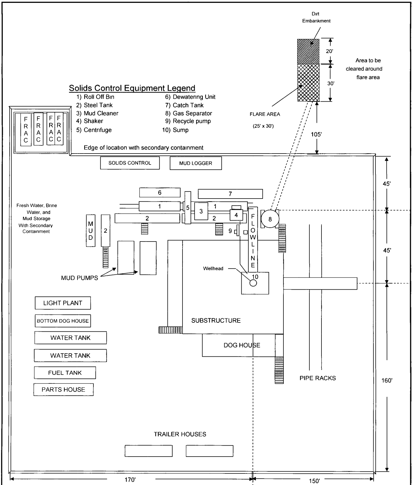
POKER LAKE UNIT 321H TYPICAL RIG LAYOUT SCHEMATIC INCLUSIVE OF CLOSED-LOOP DESIGN PLAN
