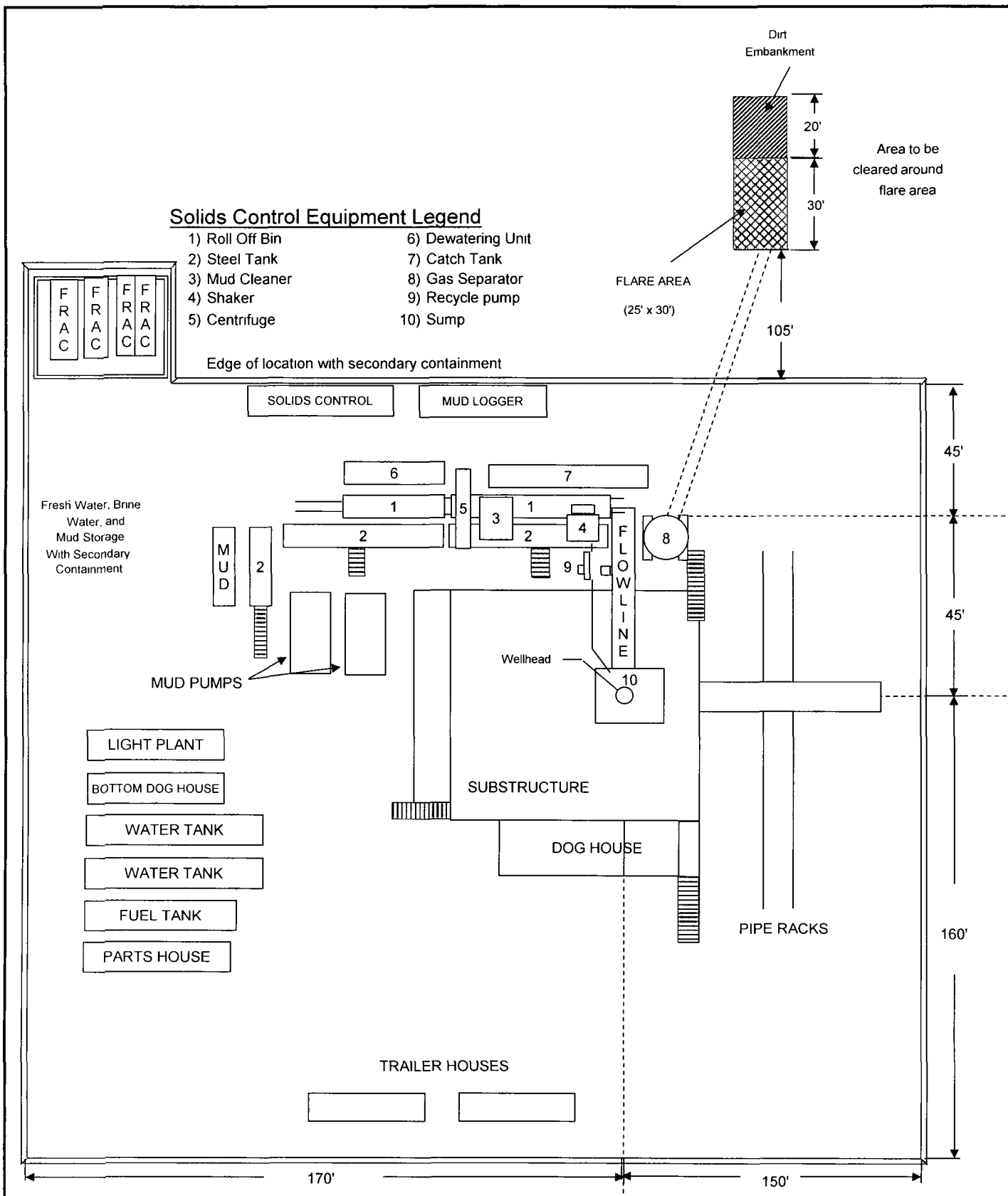
POKER LAKE UNIT 367H TYPICAL RIG LAYOUT SCHEMATIC INCLUSIVE OF CLOSED-LOOP DESIGN PLAN
