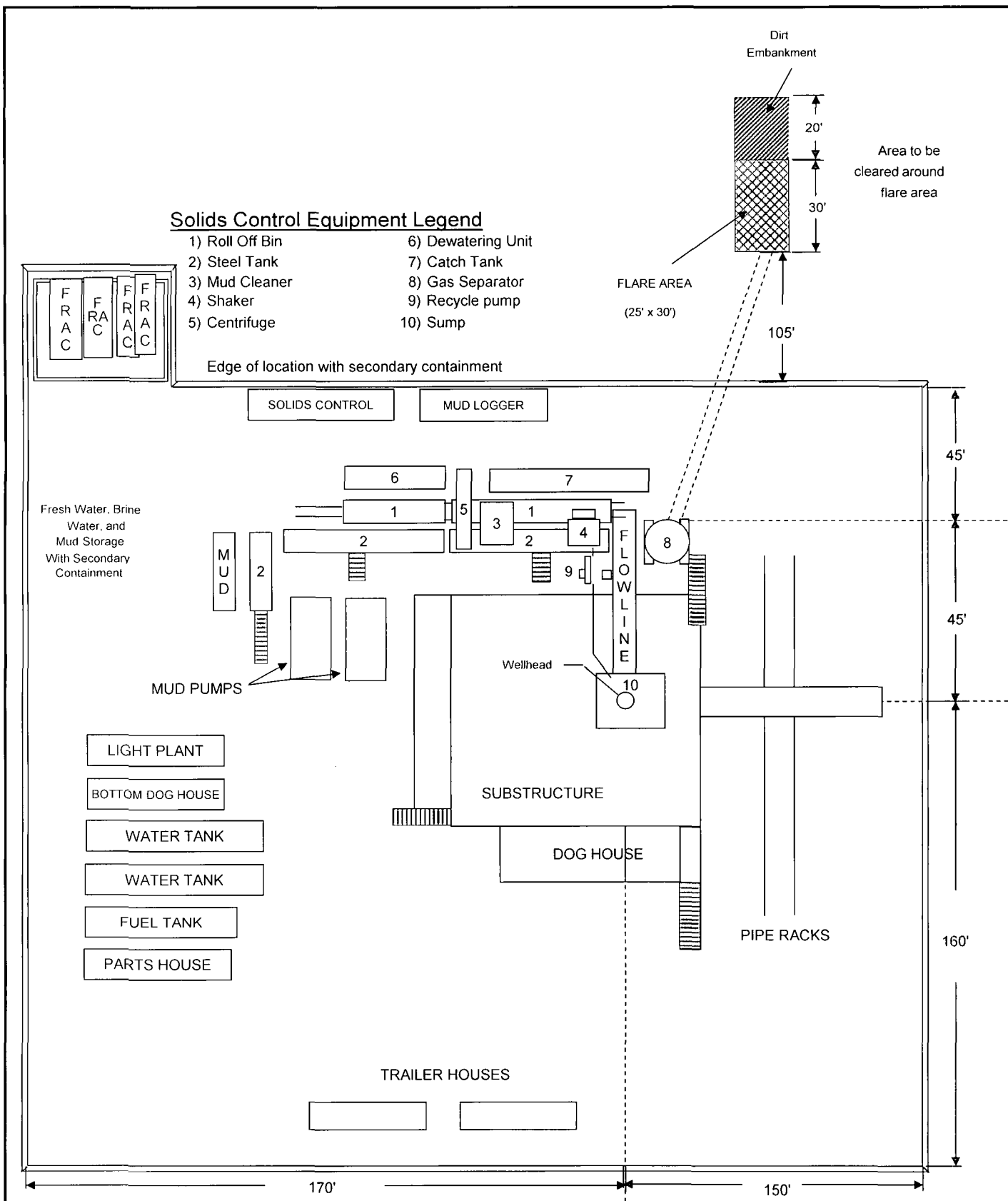
North Indian Flats 13, Well 1 TYPICAL RIG LAYOUT SCHEMATIC INCLUSIVE OF CLOSED-LOOP DESIGN PLAN
