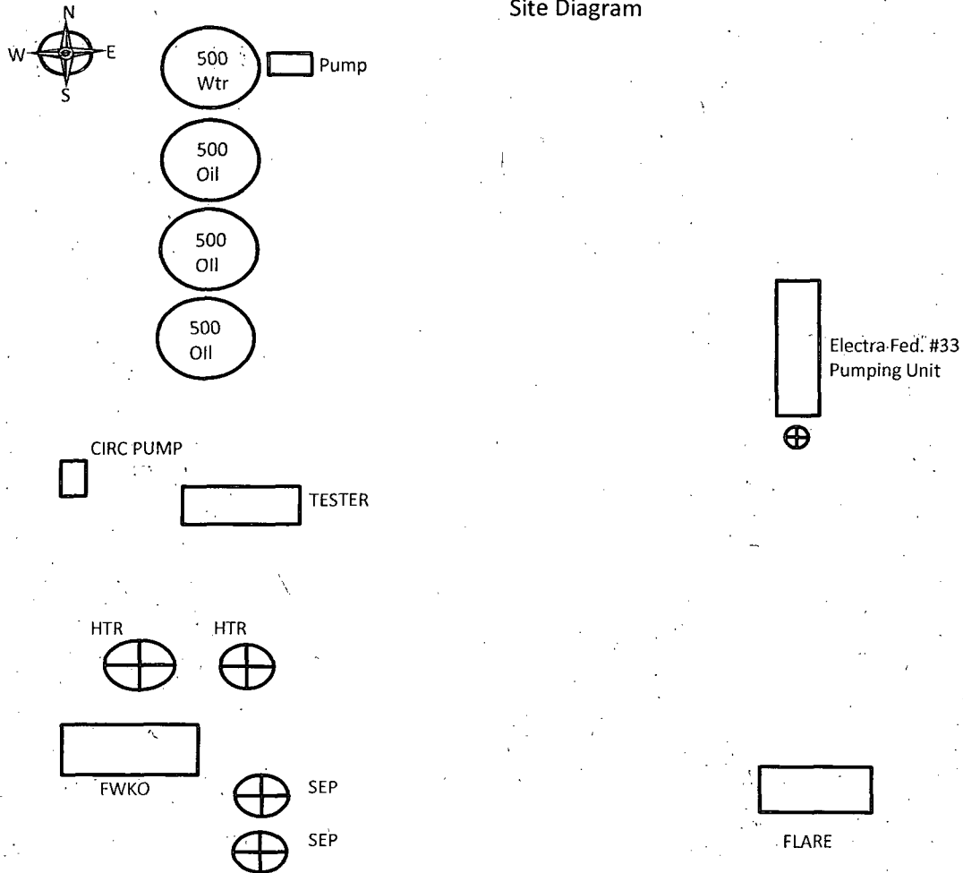
Site Diagram
