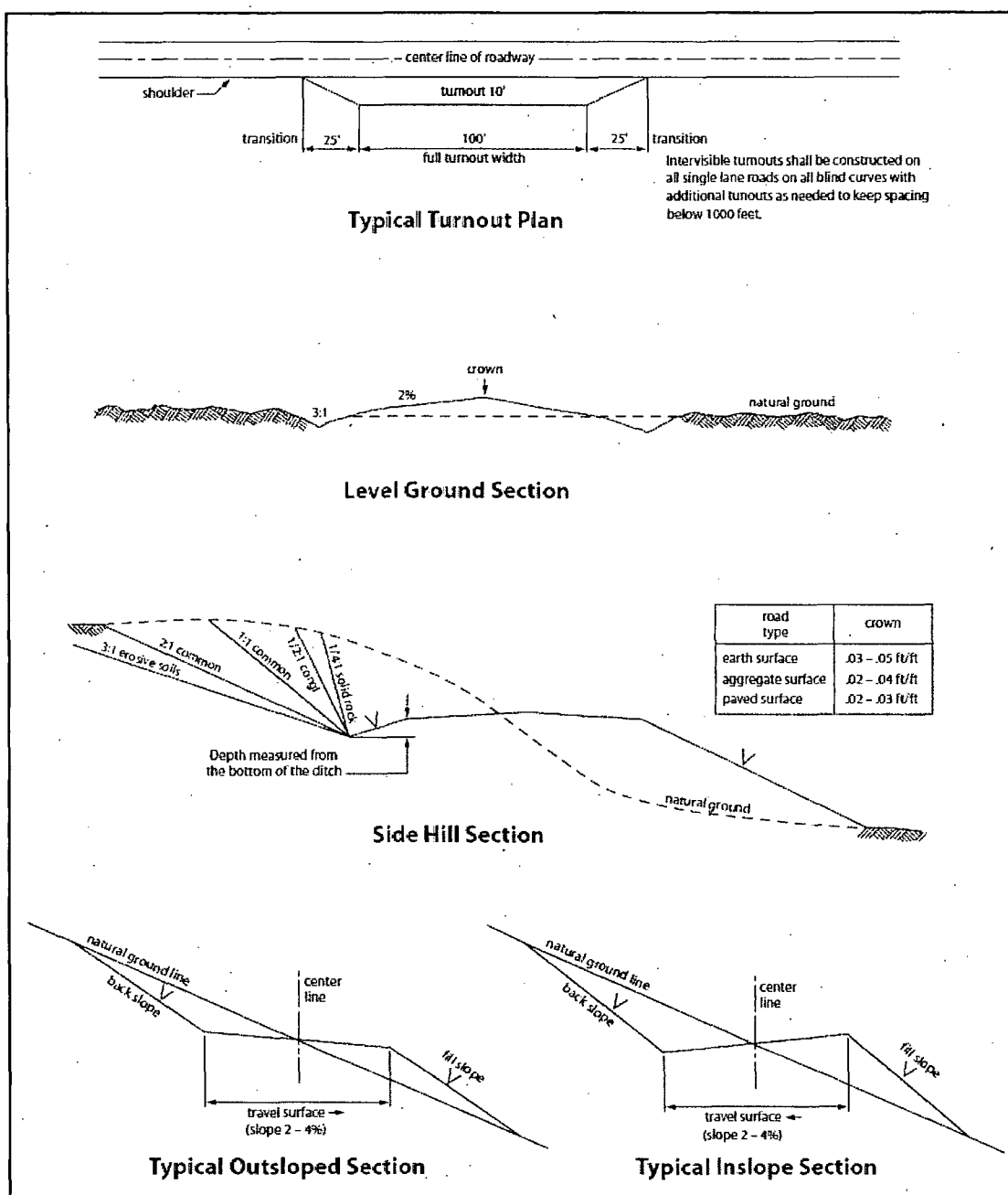
I. Figure 1. Cross-sections and plans for typical road sections representative of BLM resource or FS local and higher-class roads.
