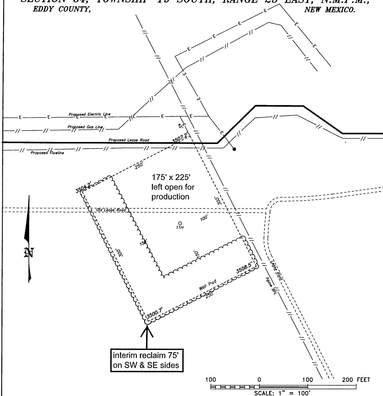
INTERIM RECLAMATION DIAGRAM (production equipment at 3H pad)
