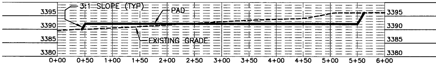
SECTION C-C'
