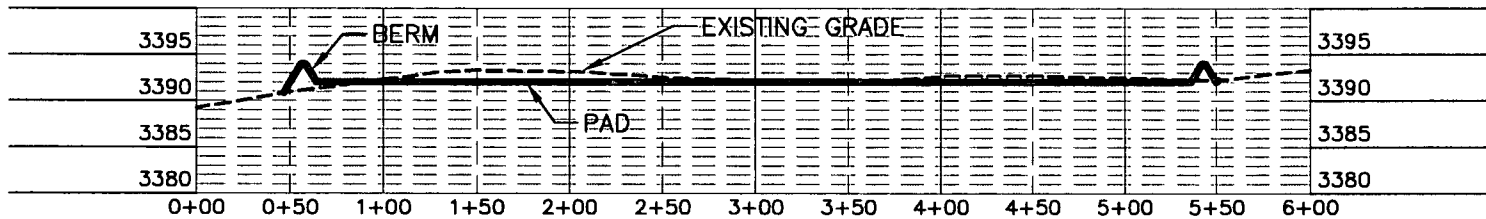
SECTION B-B'
