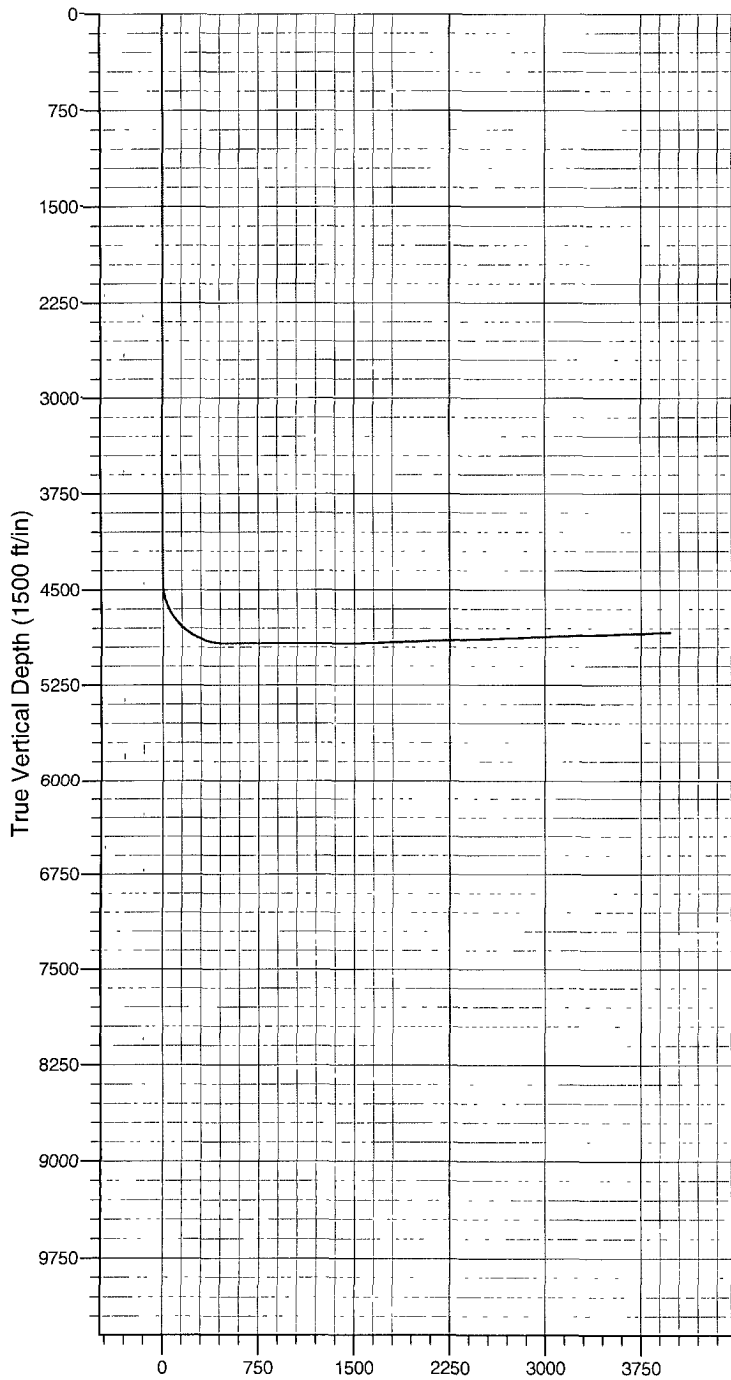
Vertical Section at 269.93° (1500 ft/in)
