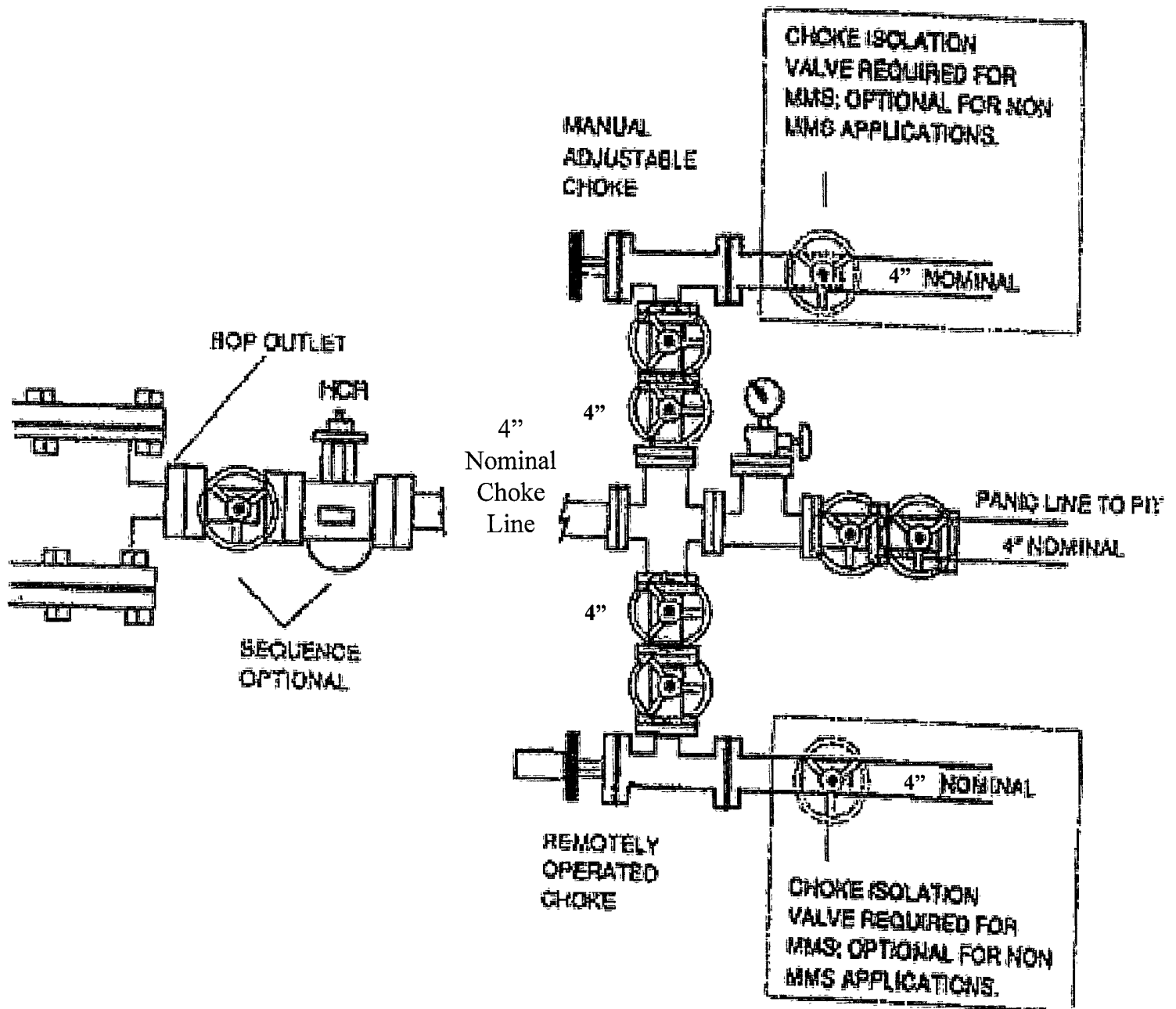
Exhibit E-1 – Choke Manifold Diagram White City 14 Federal No. 5 Cimarex Energy Co. of Colorado 14-25S-26E SHL 330' FNL & 1980' FEL BHL 2310' FNL & 1980' FEL Eddy County, NM
