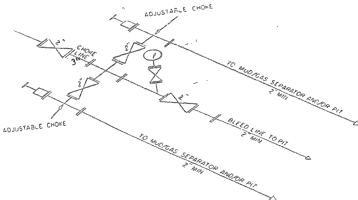
2M CHOKE MANIFOLD EQUIPMENT — CONFIGURATION OF CHOKES MAY VARY
