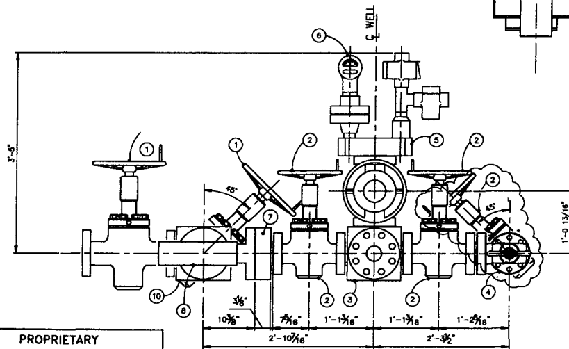
ELEVATION VIEW
