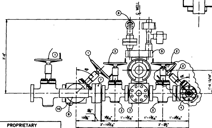
ELEVATION VIEW
