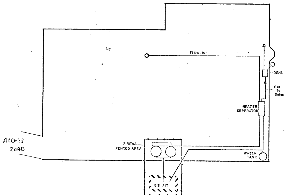
TANK BATTERY LAYOUT Scale: 1 inch = 50 Feet
