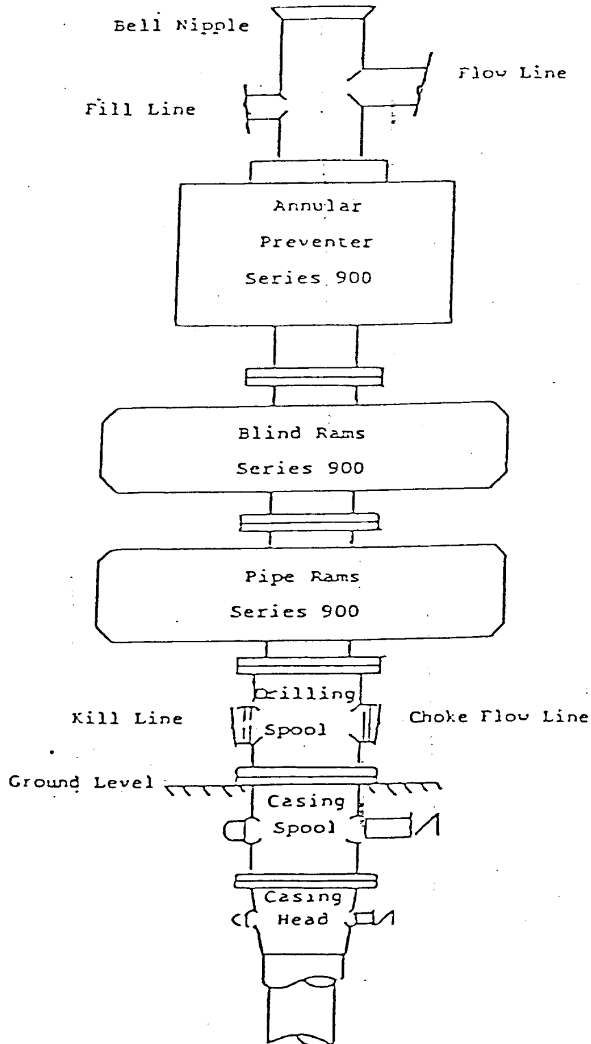
BLOWOUT PREVENTER STACK 3000# WP
