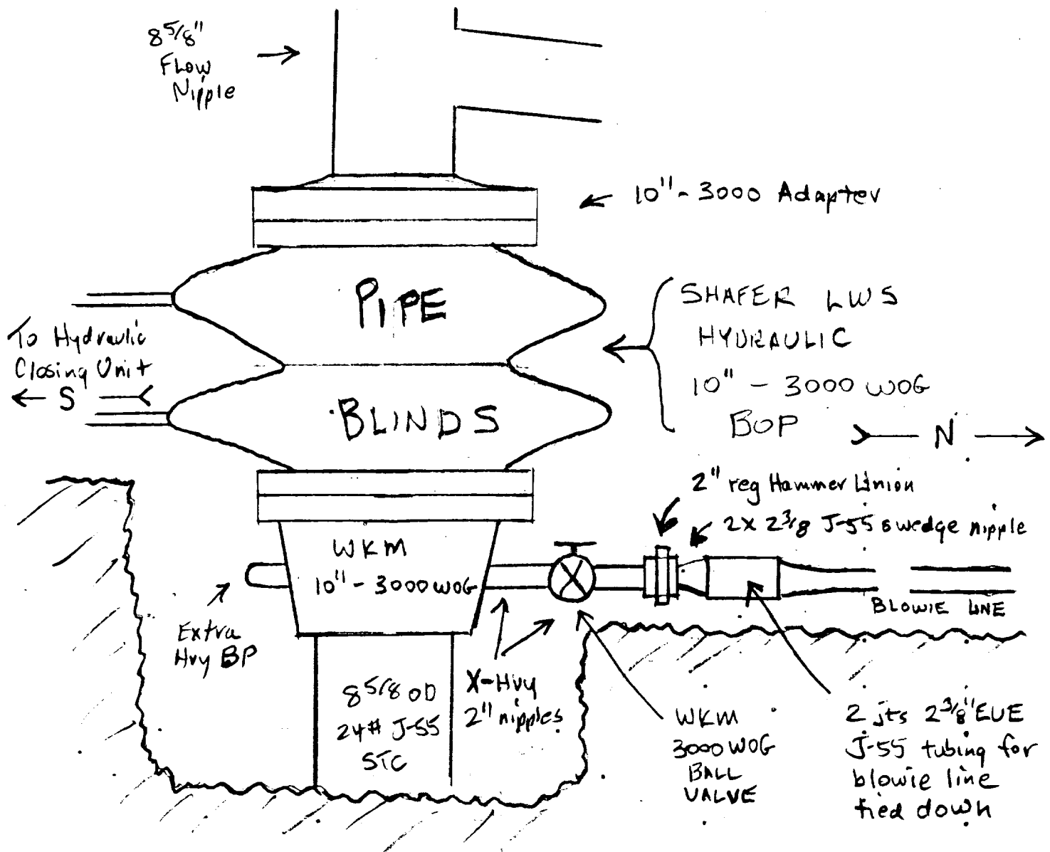
BOP Sketch
