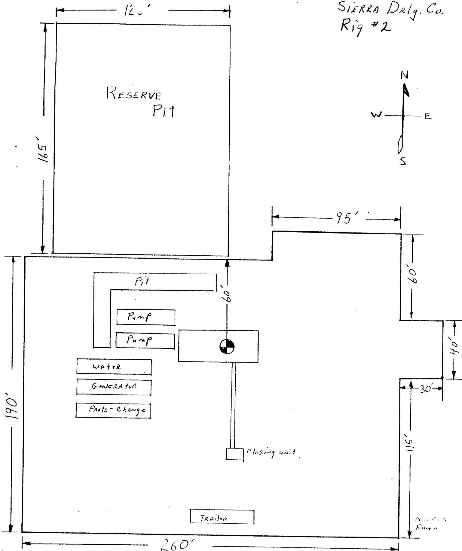
EXHIBIT "D" READ & STEVENS, INC. Langley Federal Comm., Well No. 3 Rig Layout
