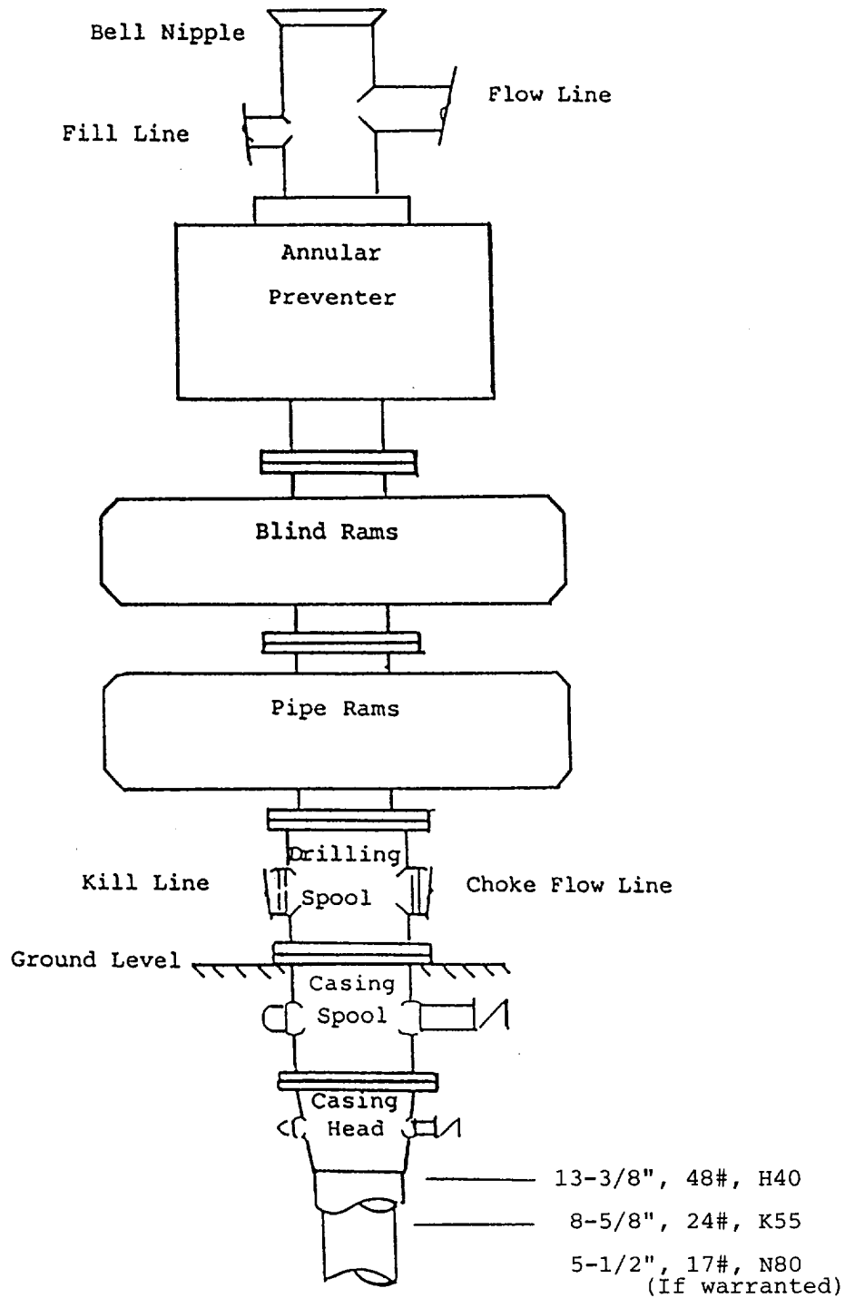
BOP DIAGRAM
