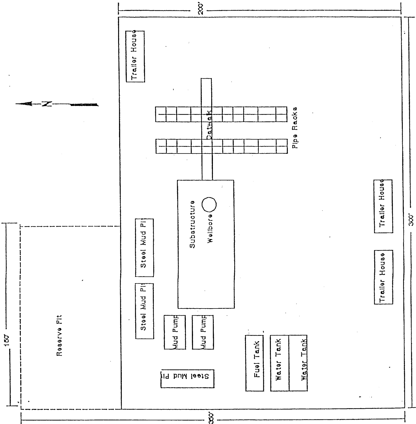
EXHIBIT 5 WELL SITE LAYOUT SANTA FE SNYDER CORP. Stock Tank "22" Fed No.1 1650' FNL & 660' FWL Section 22, T-15-S, R-28-E Chaves County, New Mexico
