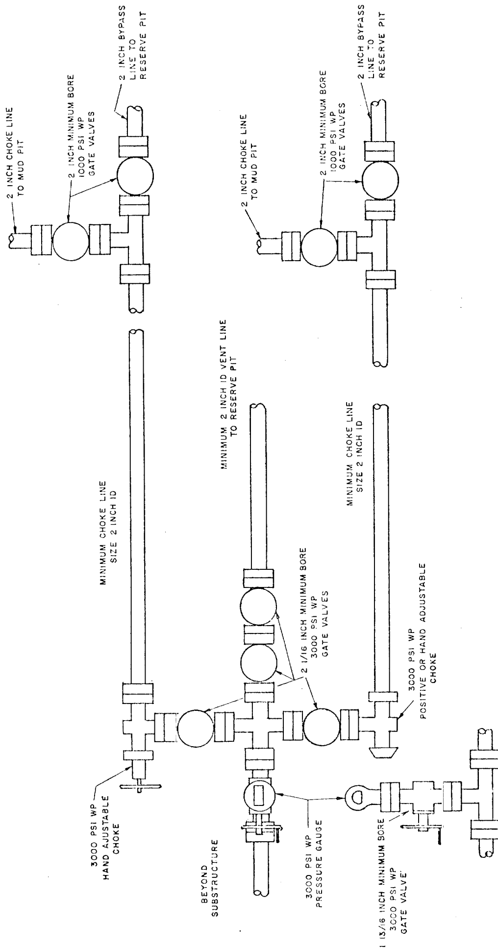
TEXAS PACIFIC OIL COMPANY CLASS II - A SYSTEM 3000 PSI WORKING PRESSURE CHOKE MANIFOLD MINIMUM REQUIREMENTS
