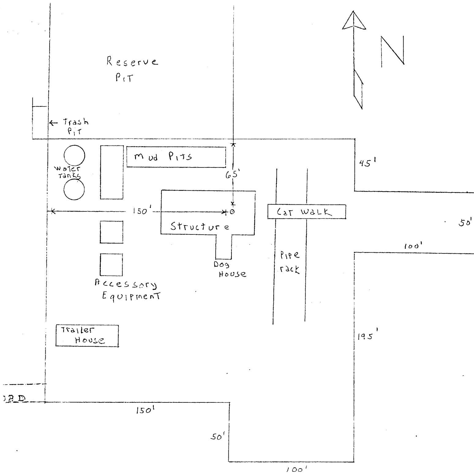
EXHIBIT "C" Callaway Fed #2 Sec 6 T16S, R28E Eddy Co, New Mexico Drilling Pad Layout
