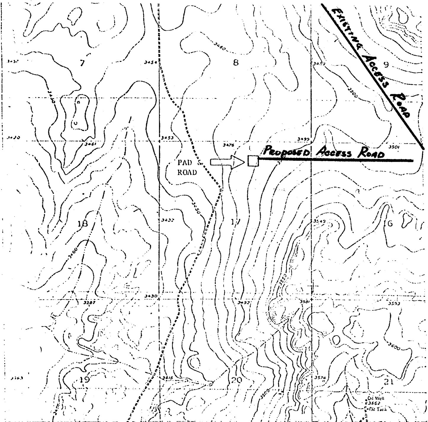
Figure 6: Location of Husky Oil Federal No. 1 and Road Sections 17 & 16, T16S, R27E, Eddy County
