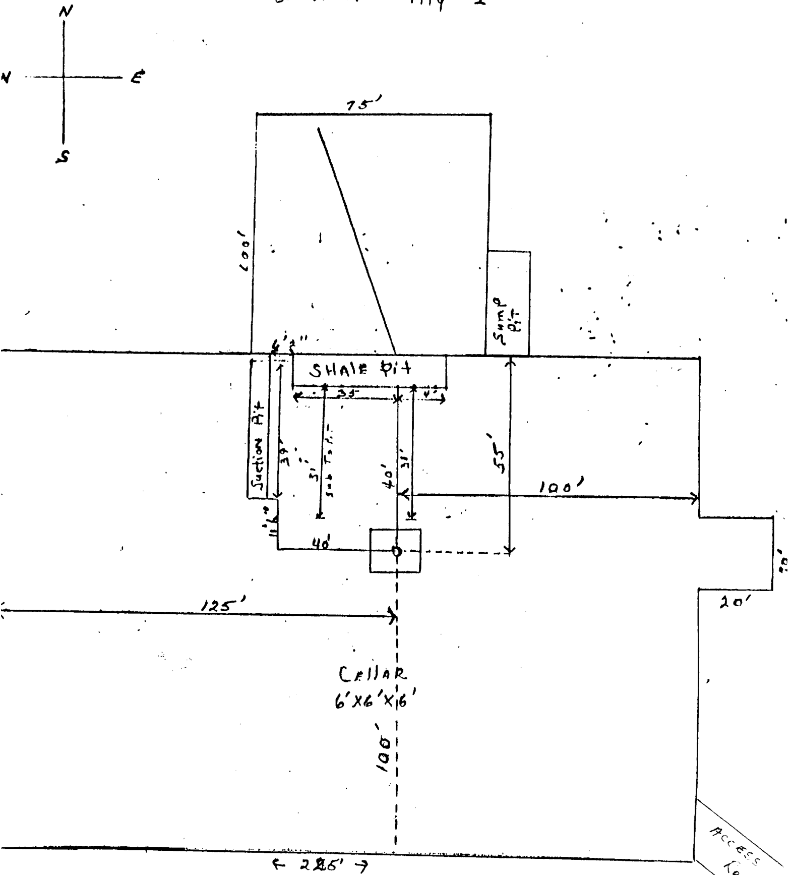
EXHIBIT "D" SNOW OIL & GAS, INC. Duffield Federal Com., Well No. 2 Pad & Pit Layout
