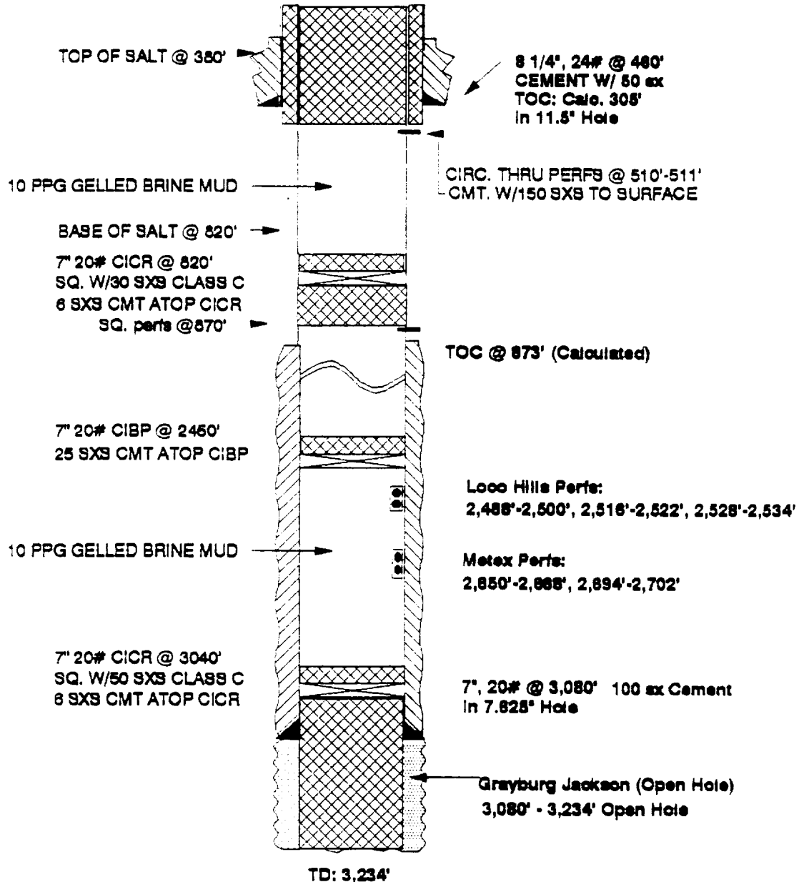
PROPOSED P&A CONFIGURATION
