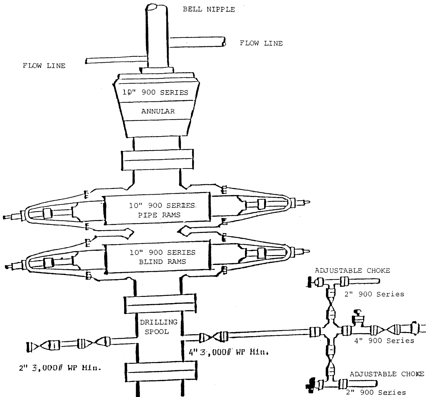
BOP & Choke Manifold Schematic Mewbourne Oil Company Empire "18" State #3 Section 18/17S/29E Eddy County, New Mexico
