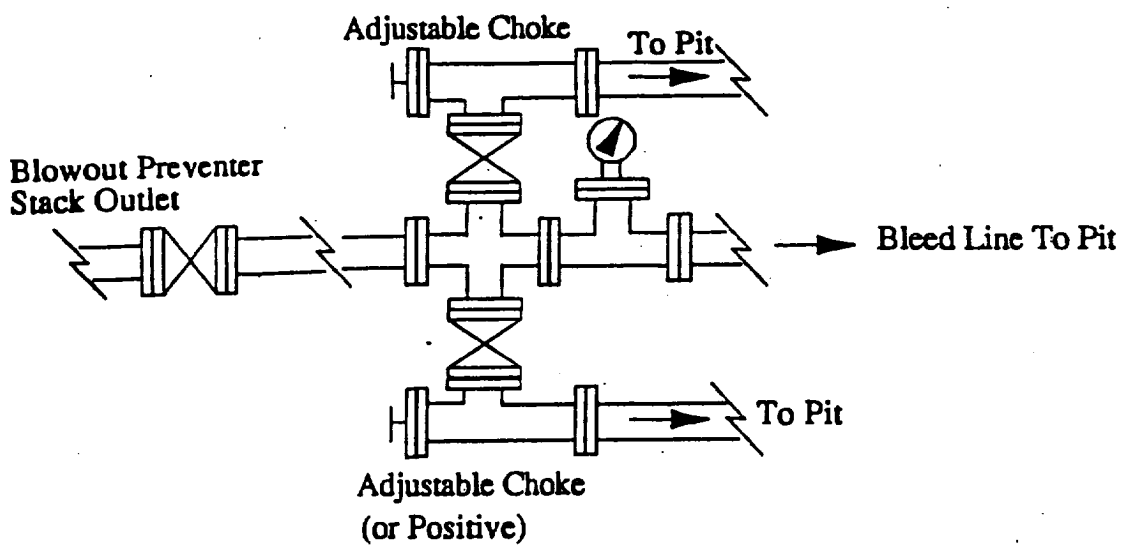
Choke Manifold
