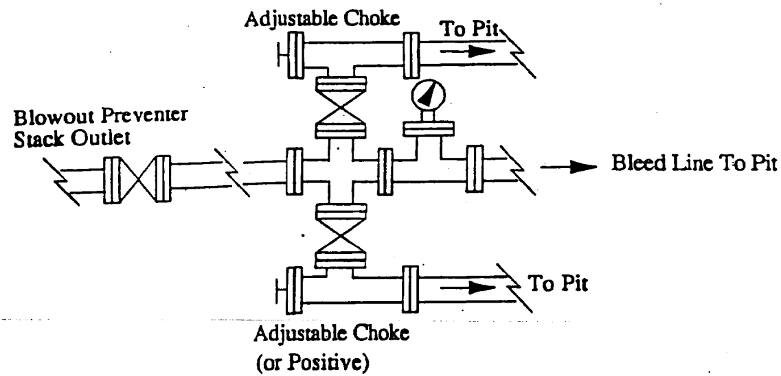
Choke Manifold
