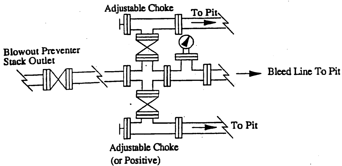
Choke Manifold
