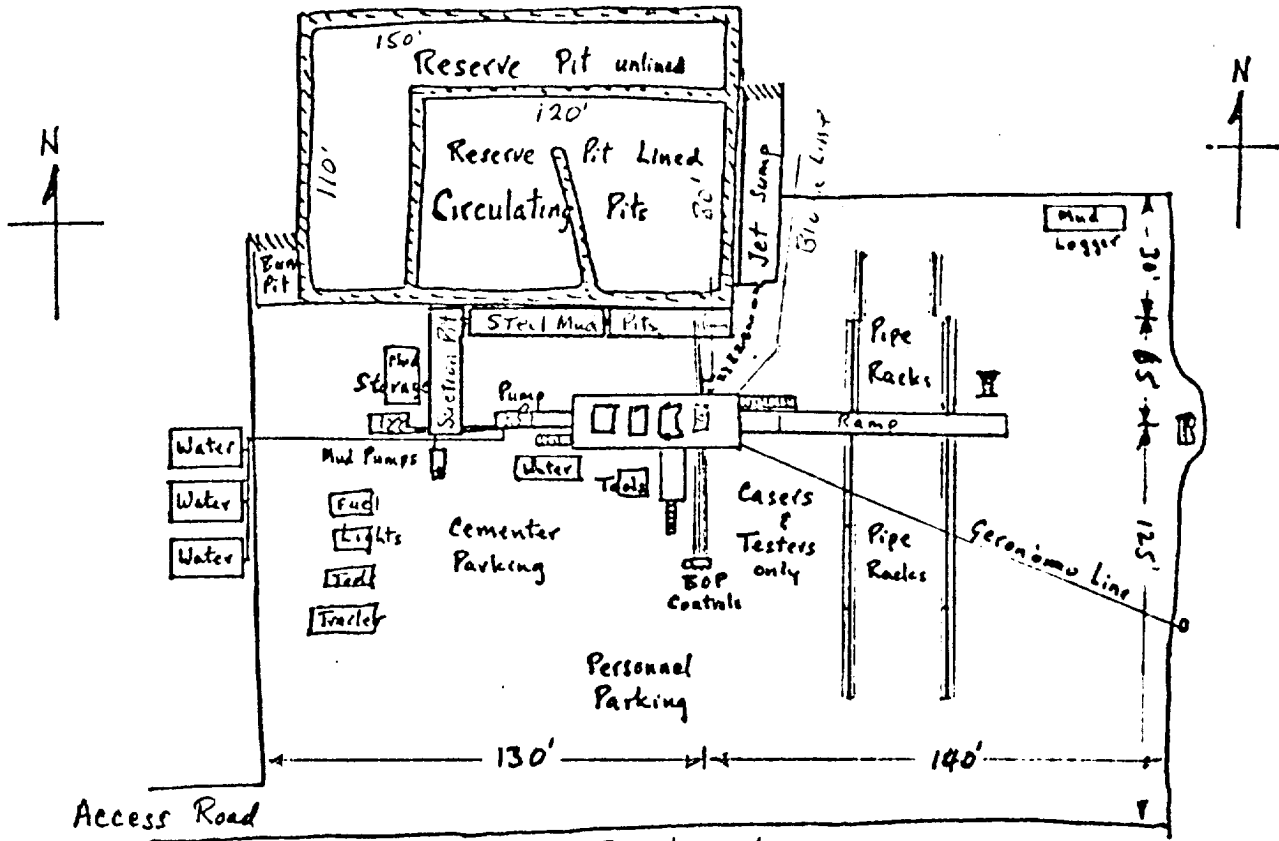
Drilling Rig Layout
