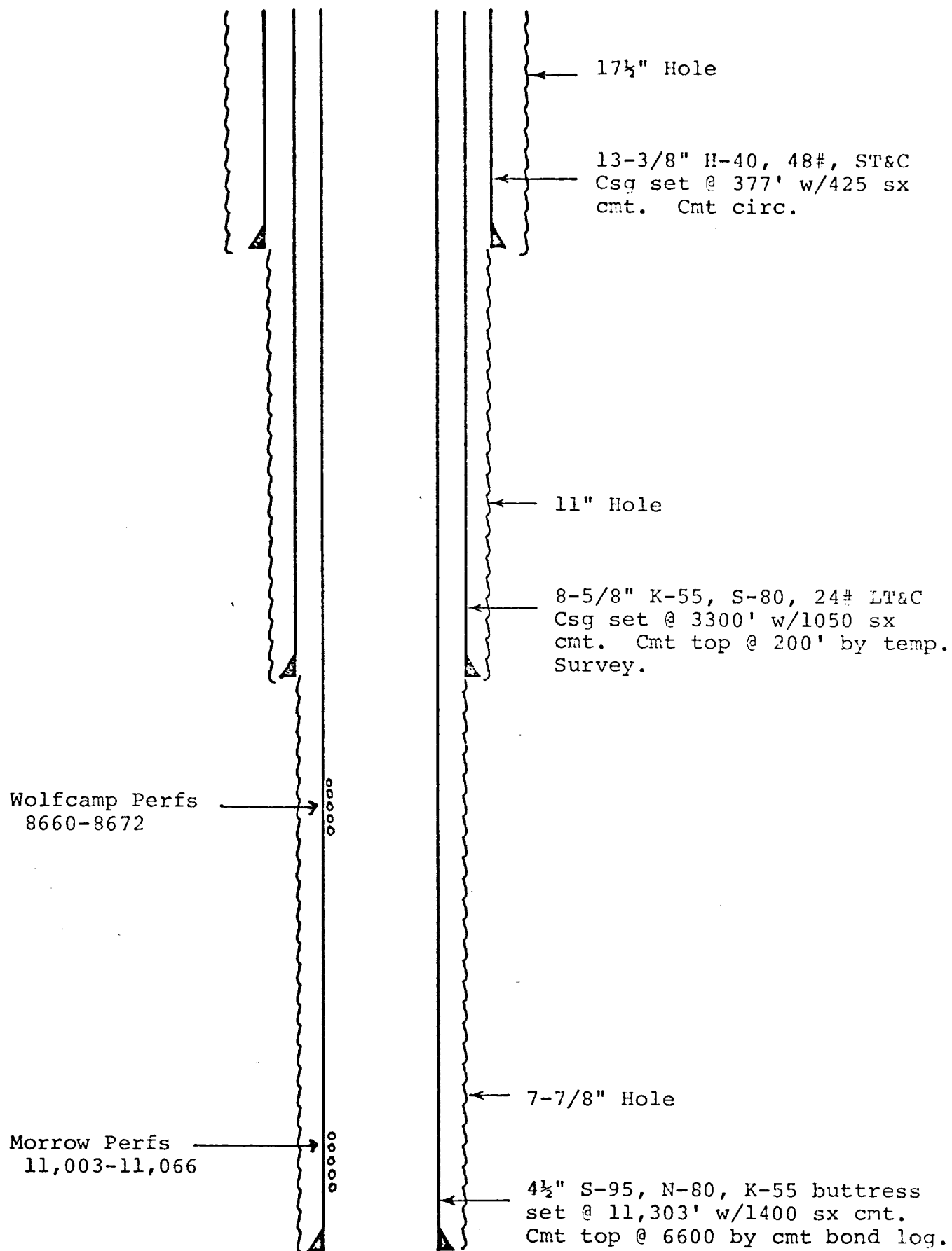
WELL BORE DIAGRAM AZTEC NO. I PALMILLO-STATE COMM.
