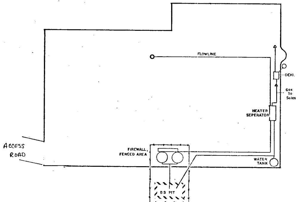
TANK BATTERY LAYOUT Scale: 1 inch = 50 Feet
