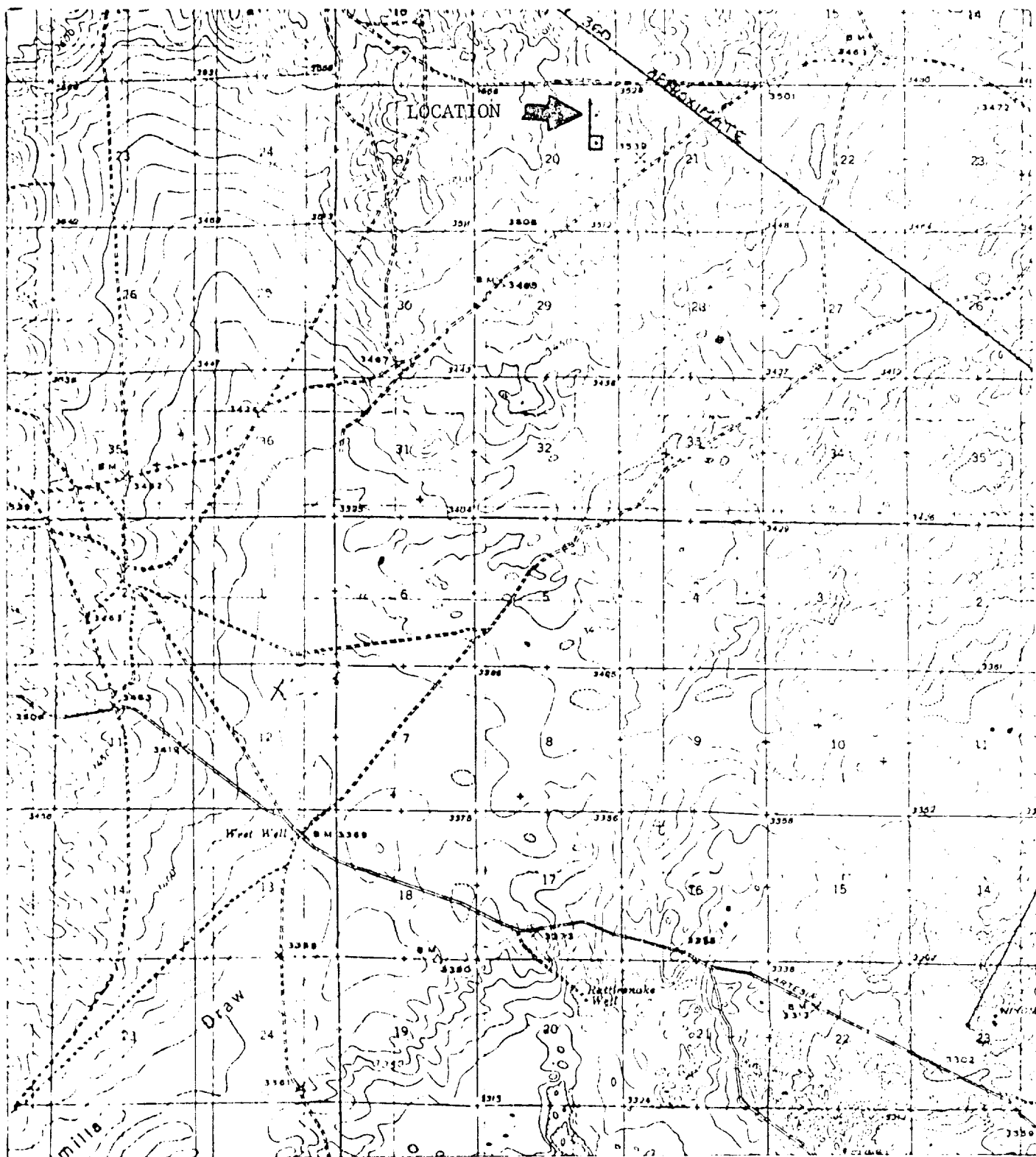
Figure 2: Location of Southland Royalty Empire Fed. 20 No. 1 Section 20, T18S, R29E, Eddy County
