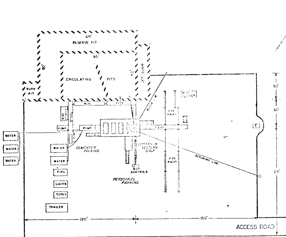
DRILLING RIG LAYOUT
