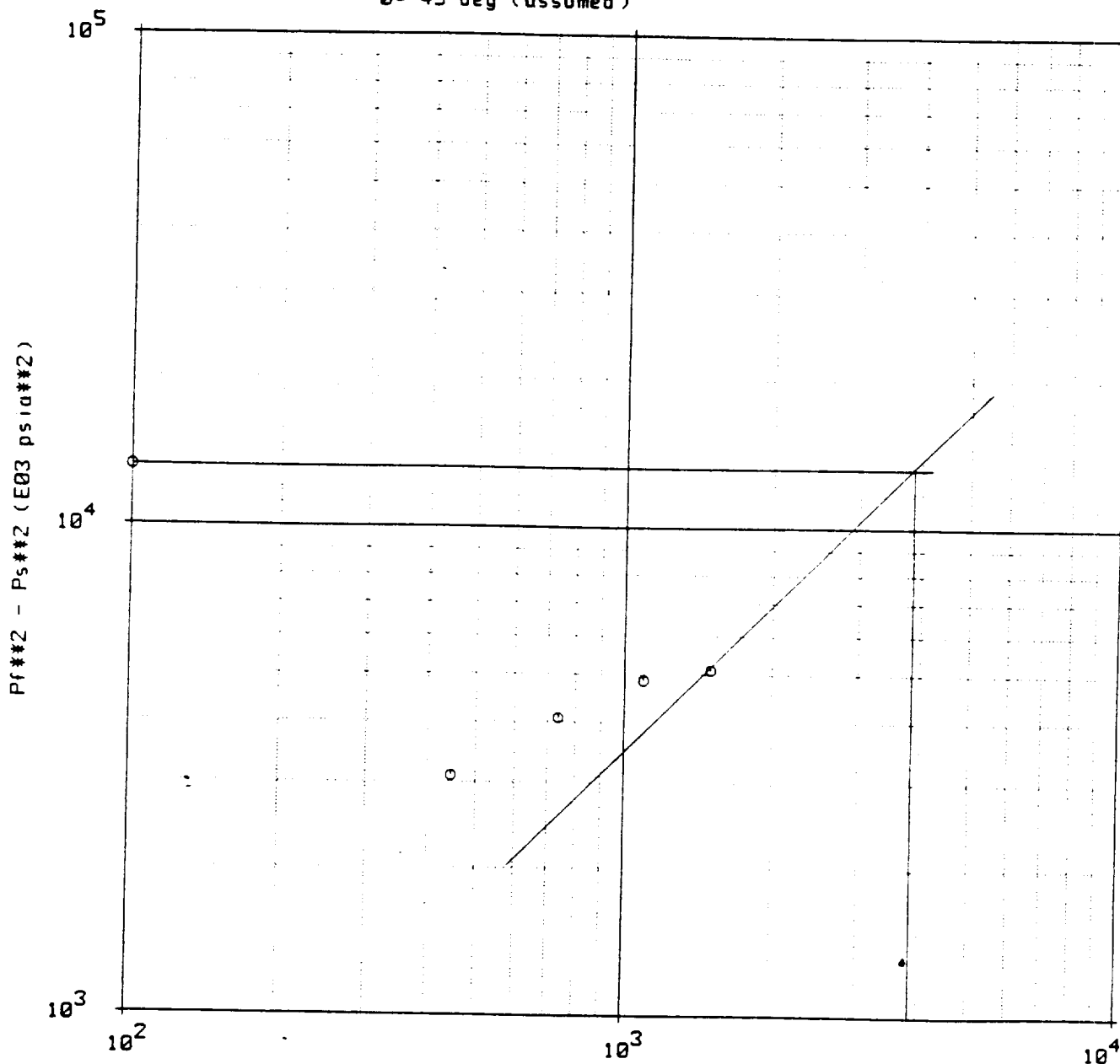
SANDFACE DELIVERABILITY PLOT Test run on 2-July-1987
